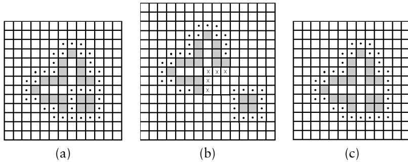
Figure 1. Two potential 2,3/3 oscillators (period = 1) are shown in (a) with the boundaries indicated by the dotted cells. If we separate the two forms (b) we find that the lower form is indeed an oscillator, but the upper form changes its behavior and starts to disintegrate. This change initiates along the boundary portion indicated by “x”, which hence is not an inert boundary and the upper shape alone is not an oscillator. But in (c) we note that the boundary is inert, hence the form within this boundary is an oscillator.
