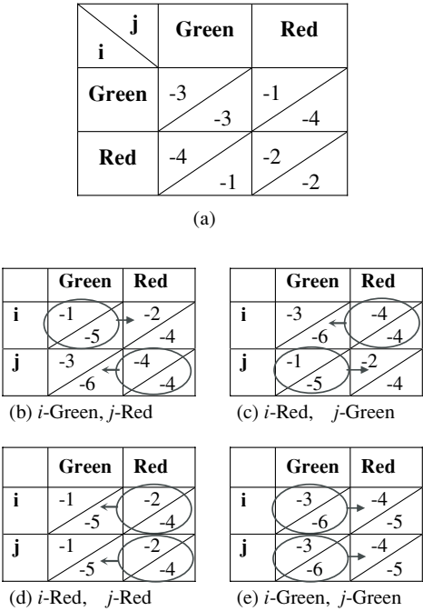
Figure 9. The LEF is inconsistent with the GEF = \sum E_{LEF} in a 2-node-linked graph of a 2-coloring problem. (a) LEF values for node i (upper) and j (lower). For example, if i is Green and j is Red, the LEF value of i is -1, and the LEF value of j is -4. (b) through (e) are LEF values (upper) and GEF values (lower) of each configuration for nodes i and j . → is the tendency to change color given the other node’s color according to the LEF judgment. → is the tendency to change color given the other node’s color according to the GEF judgment. (d) is the Nash equilibrium of the LEF methods, and (e) is the local optimum of the GEF methods. In (b) and (c), the LEF and the GEF lead the system to evolve to different configurations. So they are inconsistent even though the GEF is the sum of the LEFs of all agents. If we see “Green” as “Cooperative” and “Red” as “Defective” (a) is actually the payoff matrix of the prisoner dilemma problem [7] which is one of the most interesting problems in game theory, and the LEF of each agent is the utility function of each player.
