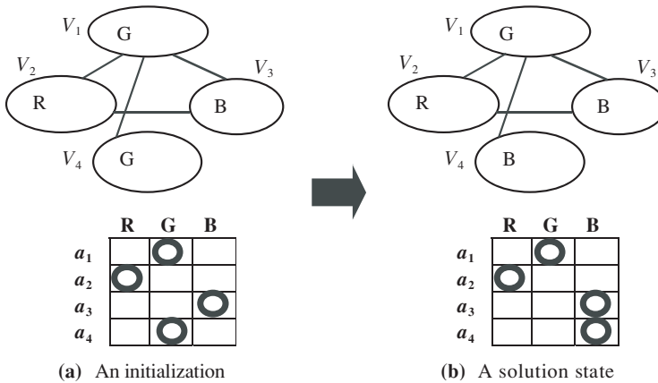
Figure 4. The MAS representation for a 3-coloring problem.
