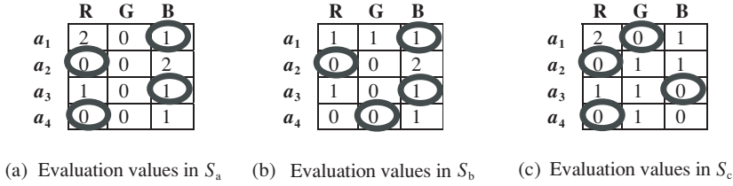
Figure 6. An example of using an LEF for the 3-coloring problem shown in Figure 5. Numbers on each row of the lattices represent the evaluation values based on equation (3) for an agent's three possible states (colors): R, G, or B. Circles refer to the current state of the agent. (c) shows that S_c is a solution state because all agents are in nonconflicting states. From S_a , if a_1 moves first, it will most probably change its state from B to G and get to S_c . If a_4 moves first, it will stay, or with small probability, it will change to G and get to S_b .
