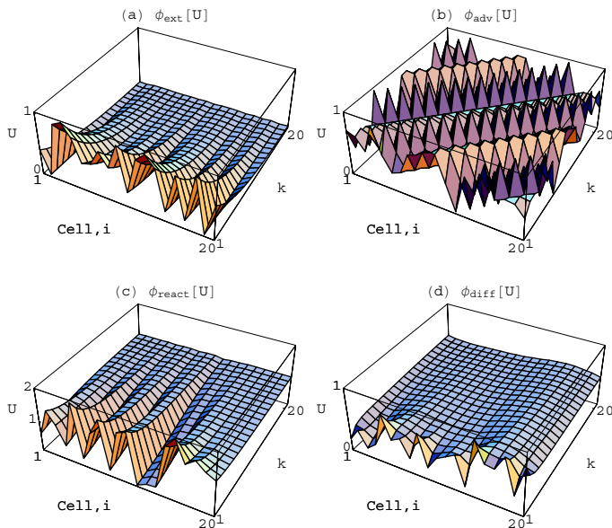
Figure 4. Examination of the elementary transport processes for a random initial distribution and wrapped boundaries. (a) External interaction, H = 0.1 , g = 0 ; (b) Advection, V = 1 ; (c) Logistic reaction kinetics, equation (17), A = 0.25 , B = 1 ; (d) Diffusion, D = 0.3 .
