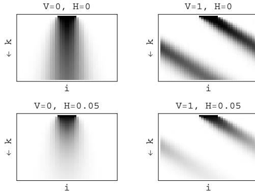
Figure 5. Examination of a multi-physics process consisting of advection, diffusion ( D = 0.25 ), and external interaction. Computed using the rule \phi_{\text{adv}}[\phi_{\text{diff}}[\phi_{\text{ext}}[U]]] for a square wave initial distribution and wrapped boundaries.
