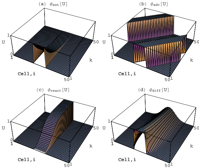
Figure 3. Examination of the elementary transport processes for a square wave initial distribution and wrapped boundaries. (a) External interaction, H = 0.1 , g = 0 ; (b) Advection, V = 1 ; (c) Logistic reaction kinetics, equation (17), A = 0.25 , B = 1 ; (d) Diffusion, D = 0.3 .
