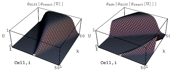
Figure 6. Examination of a multi-physics process consisting of advection, diffusion ( D = 0.25 ), and logistic growth kinetics ( A = 0.2 , B = 1 ). Computed using the rule \phi_{\text{adv}}[\phi_{\text{diff}}[\phi_{\text{react}}[U]]] for a square wave initial distribution and wrapped boundaries.
