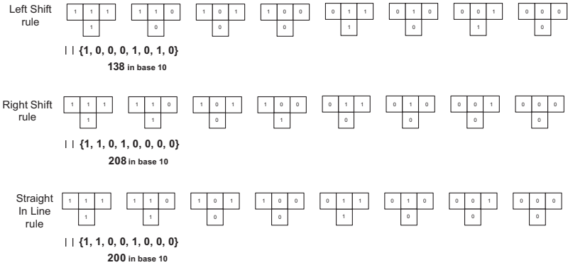
Figure 10. CA rule representation for Rows 3 through 5.
