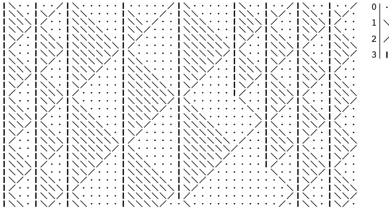
Figure 4. Decreasing sequence of subshift attractors.
