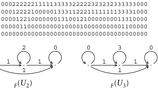
Figure 1. Intersection of attractors.
