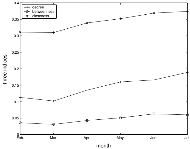
Figure 3. Degree, betweenness, and closeness indices of the new replied networks month-by-month.
