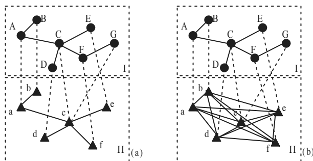
Figure 1. Example ID networks according to the relationship of replying to articles: (a) new replied network; (b) traditional replied network. (I) Replied network of one root article A and six replied articles. (II) ID network derived from the relationship of replied articles. An edge between two IDs in the new replied network indicates that opinions about a certain event are the same or different, shown as (a). For instance, although article C and G are different replied articles, they have the same ID c so there is only one edge between IDs c and f. However, an edge in the traditional network indicates that IDs enjoy the same interests on the same topic making the network shown as (b) a completed graph.
