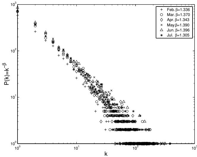
Figure 2. Degree distributions for replied networks of six months. All of them follow scale-free forms but the exponents are obviously less than 2. The range of exponents of these degree distributions is [1.3, 1.4] actually.
